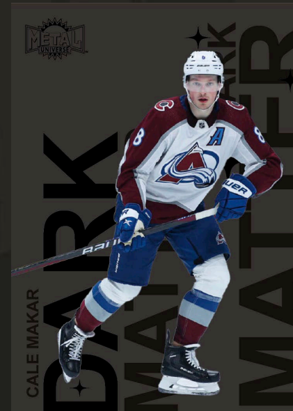
Dark Matter
