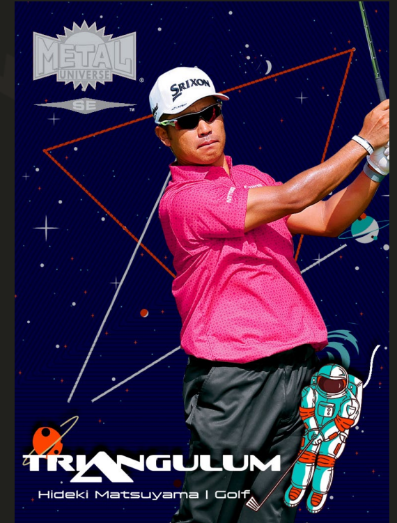
Triangulum
