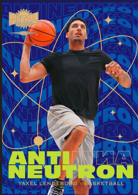
Antineutron
